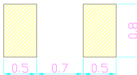
Recommended Soldering Pattern (Units : mm)
