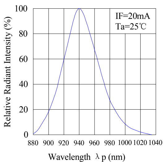
Spectral Distribution
