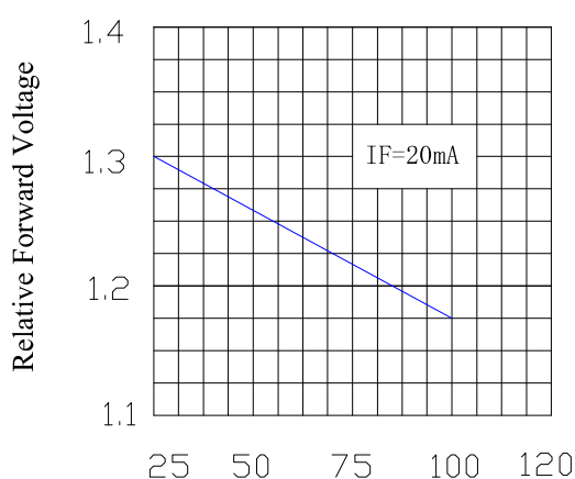
Forward Voltage & Ambient Temperature(°C)
