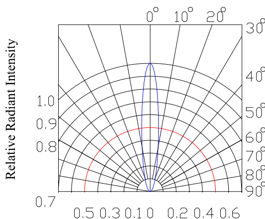
Relative Radiant Intensity & Angular Displacement
