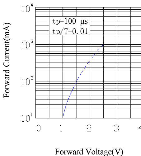
Forward Current & Forward Voltage
