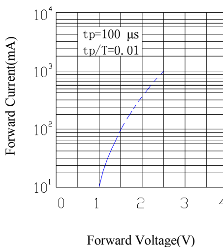
Forward Current & Forward Voltage
