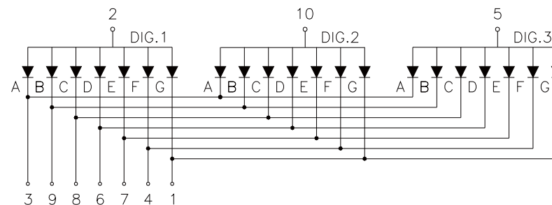
Common Anode JSD-3032Bx
