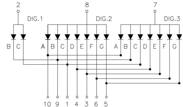
Common Anode JSD-5032Dx
