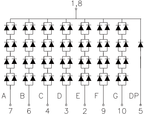
Common Anode JSD-30013Fx
